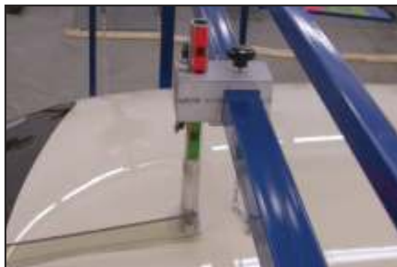
THE ROOF HEIGHT IS MEASURED BY VIEWING THE CALIBRATED ROD ATTACHED TO THE POLYCARBONATE GAUGE.
